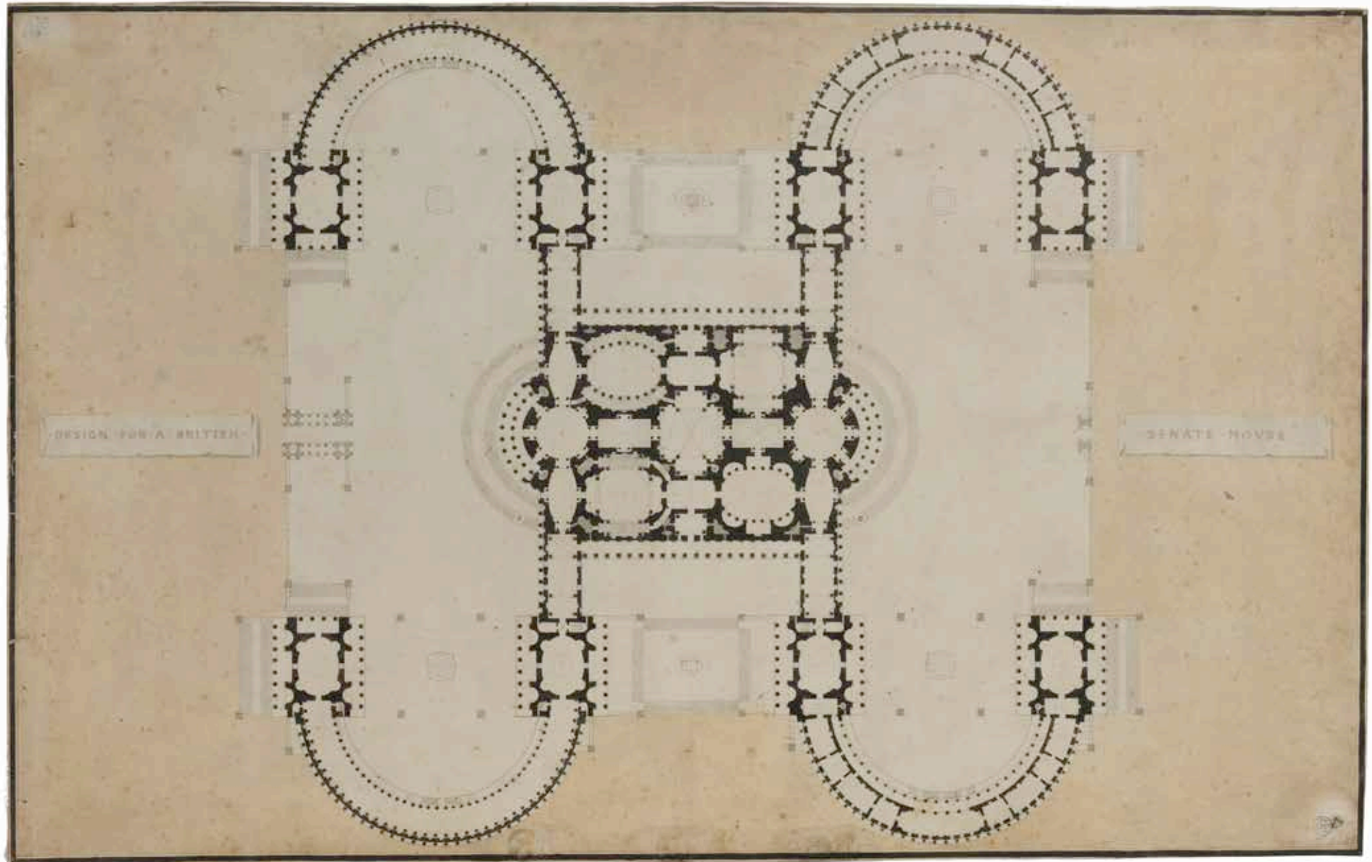
Figure 14.2 Soane's Plan for a British Senate House 1779. (SM 45/1/35). Drawing (7). From an unknown draughtsman, with 'serif-less' title blocks. © Sir John Soane's Museum, London. Photo: Hugh Kelly.
